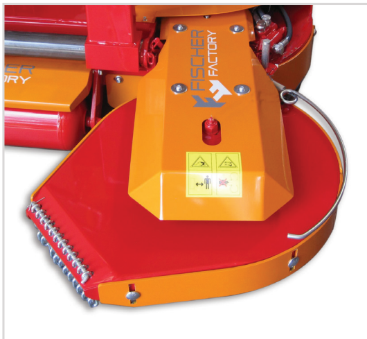
Hydraulic Sensor Rod Head (Available in 24" and 32" sizes)
