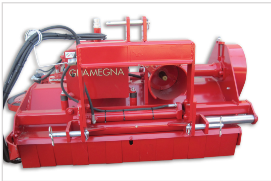
Hydraulic off-set of mower on 3-point frame to reach under vines and trees
